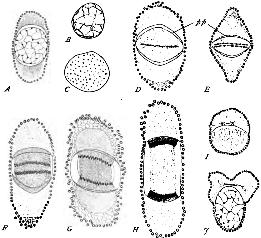
Fig. 44.—Mitosis in the rhizoped Actinosphaerium . [BRAUER.] 1
